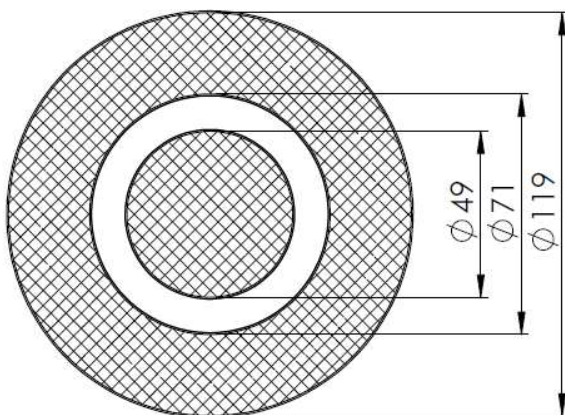
Figure 1. The gripping surface and magnetic poles of MAP-120R.
