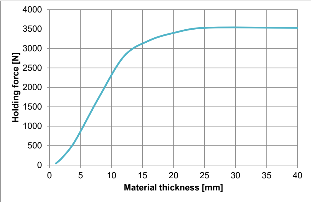
Figure 2. MAP-120R holding force in proportion to material thickness
