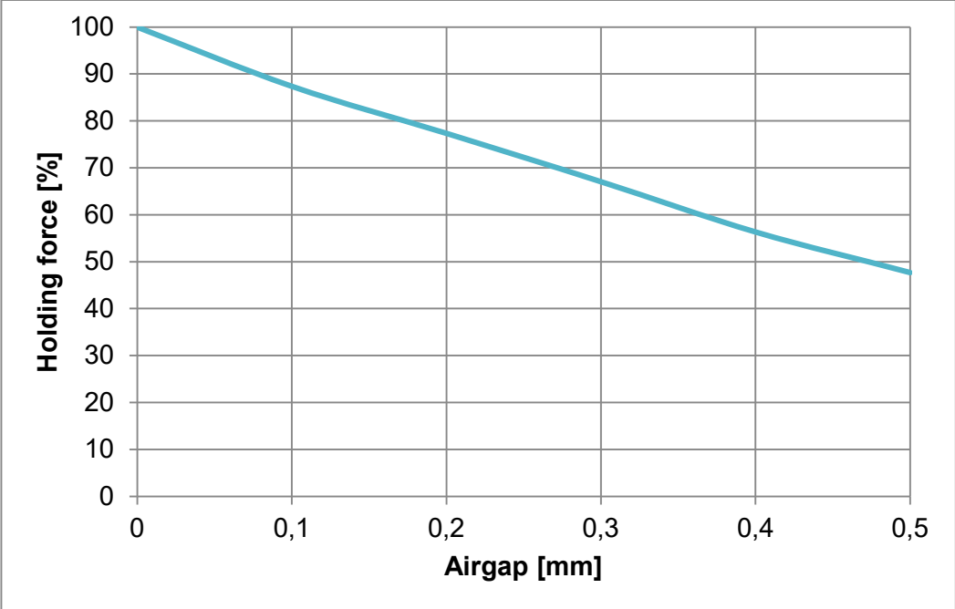
Figure 3. MAP-120R holding force in proportion to airgap
