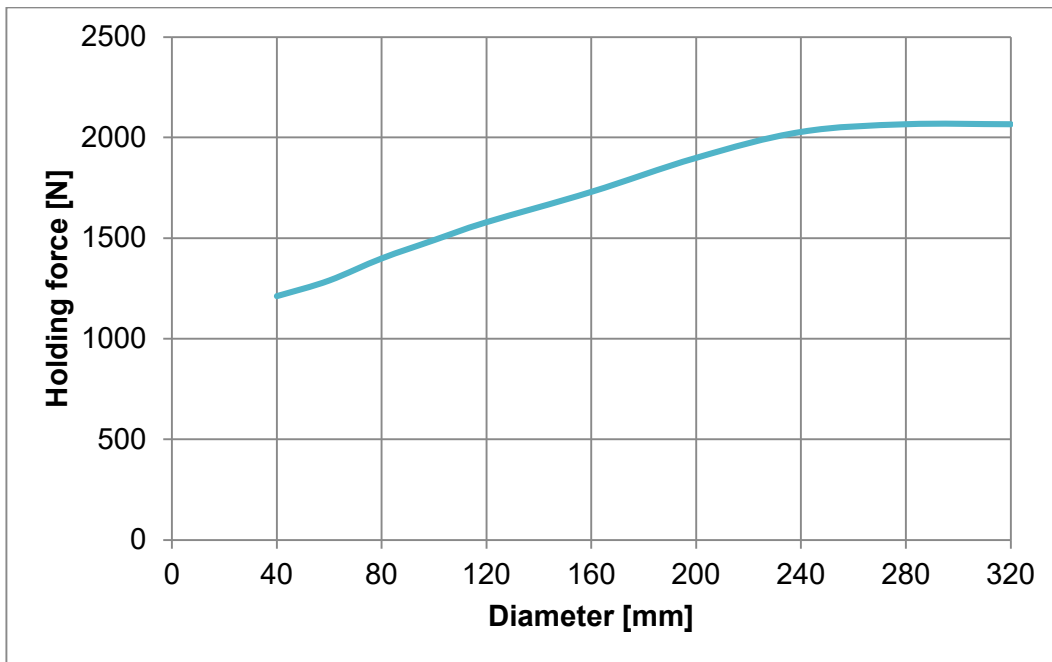
Figure 4: MAP-120R holding force in proportion to round part diameter
